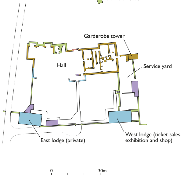
HALL PLAN
