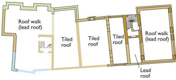
FIFTH-FLOOR PLAN
