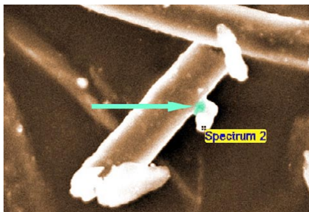
Figure 9. A Scanning Electron Microscopy image showing dust particulates cemented to textile fibres. The highlighted region binding the particle to the fibre is rich in calcium and, using Raman microspectrometry, has been identified as a fine grained calcite.
